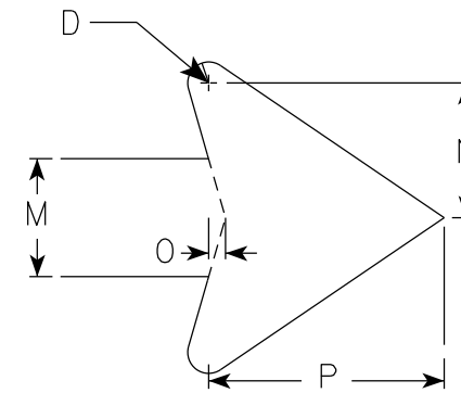
ARROW DETAIL
