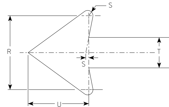
ARROW DETAIL
