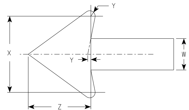
ARROW DETAIL
