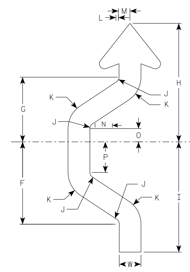
Arrow Detail
