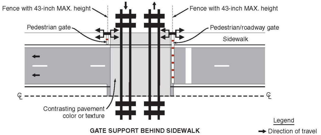
Figure 8C-7. Examples of Placement of Pedestrian Gates
