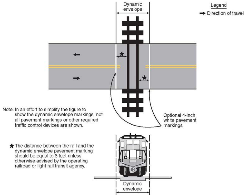
Figure 8B-9. Examples of Light Rail Transit Vehicle Dynamic Envelope Markings for Mixed-Use Alignments
