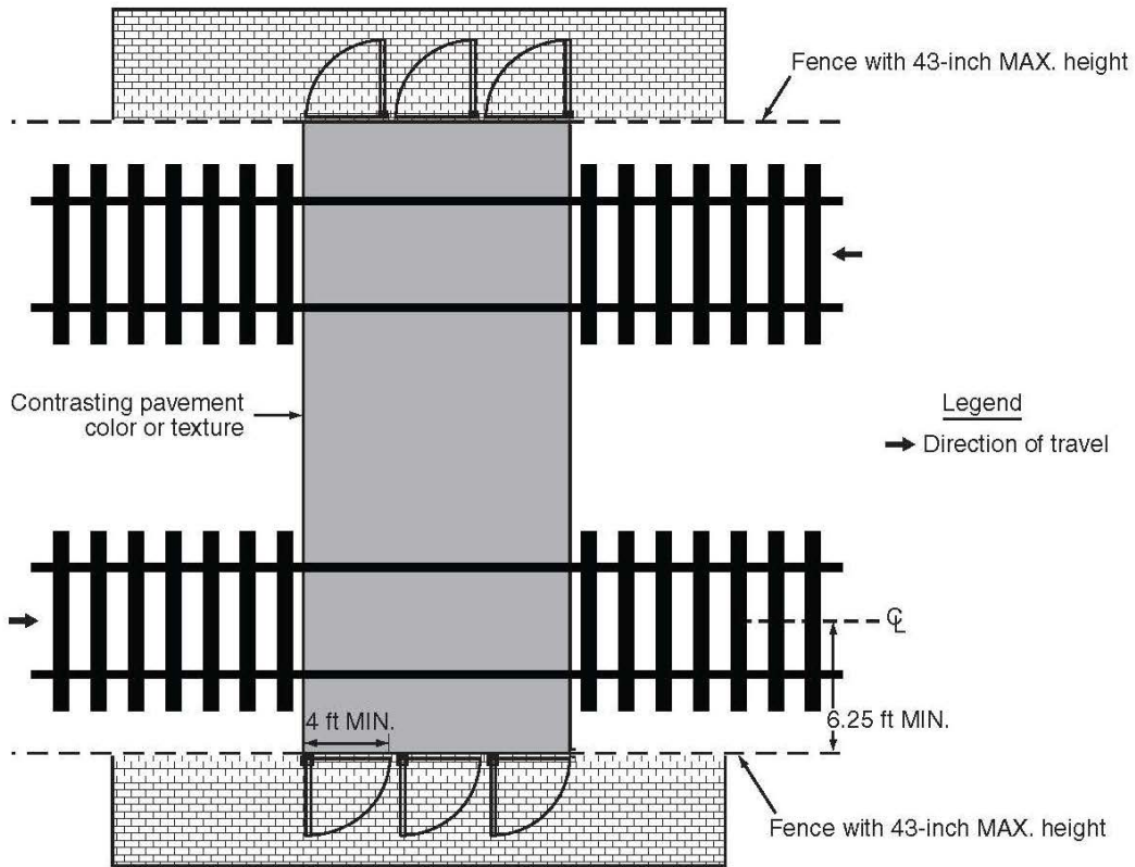
Figure 8C-8. Example of Swing Gates
