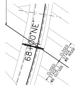
PLAN AT FIELD SPLICE 5
