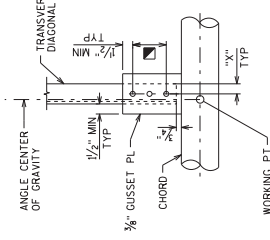
BOLTED TRANSVERSE DIAGONAL CONNECTION
