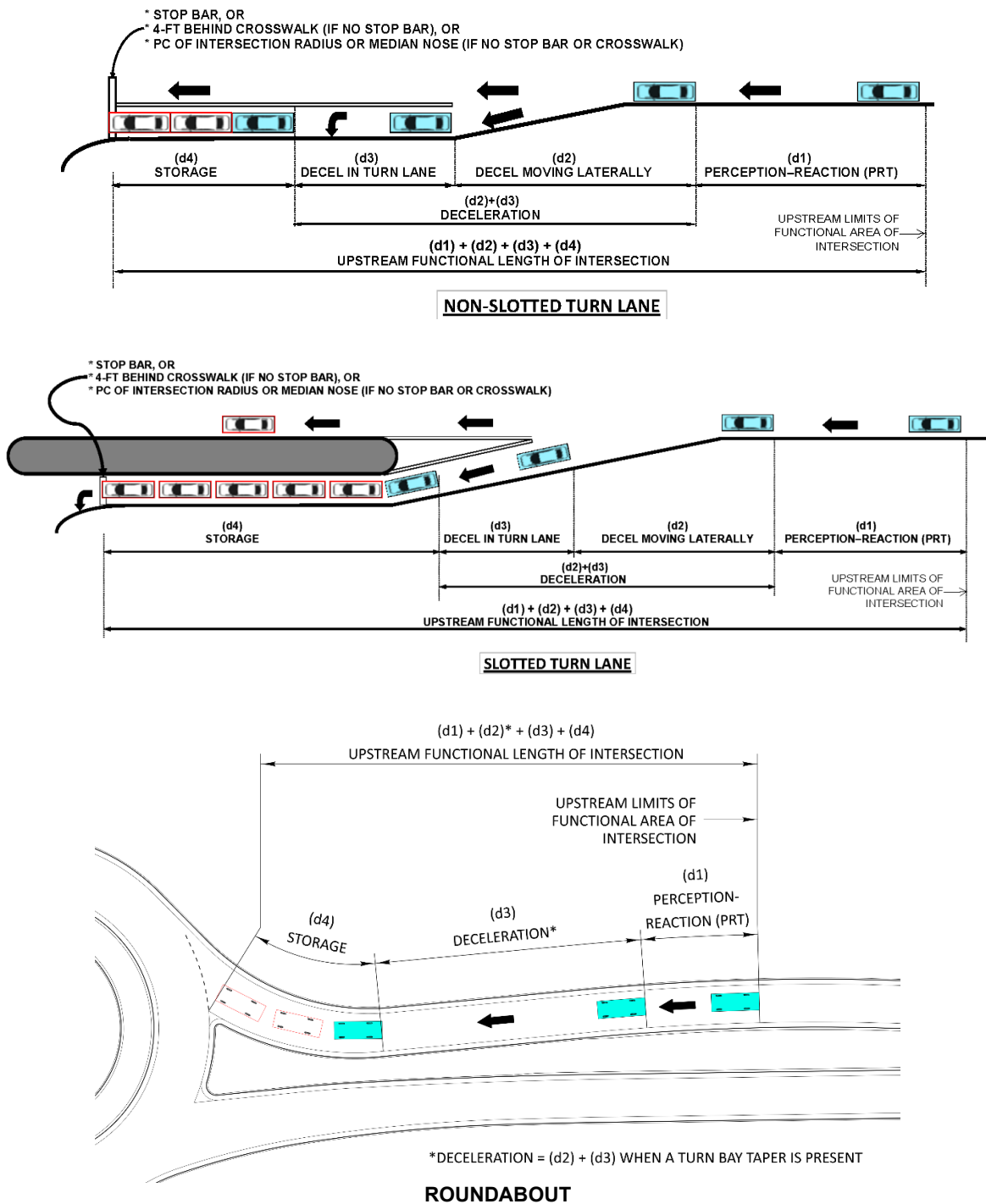
Figure 2.10 Upstream Functional Length of Intersection Elements 31
