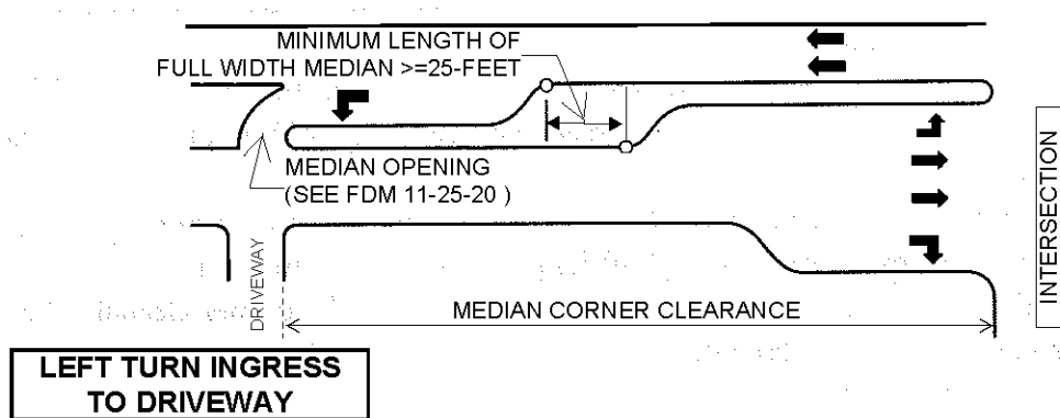
Figure 2.13 Intersection Median Corner Clearances 41
