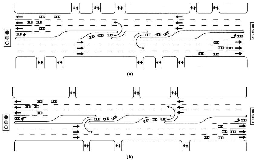
Figure 20.4 Directional Median Openings for U-turns 88 (a) Downstream from Signalized Intersection (b) Upstream from Signalized Intersection
