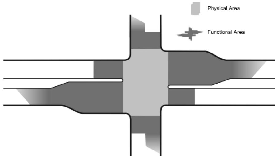
Figure 2.6 Physical and Functional Areas of a Non-roundabout Intersection 30
