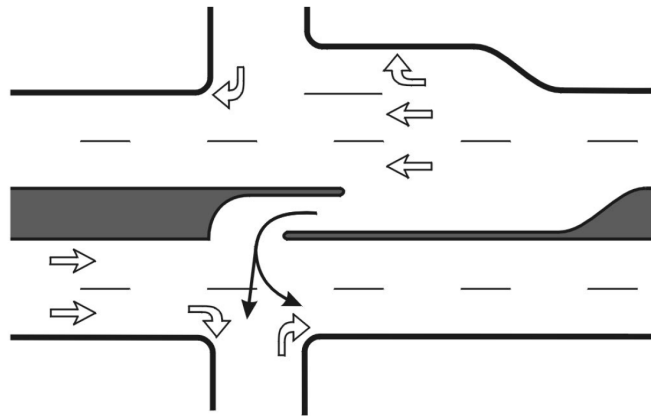
Figure 20.1 Directional Median Opening 85
