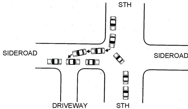
Figure 2.14 Inadequate Corner Clearance on Sideroad 42
