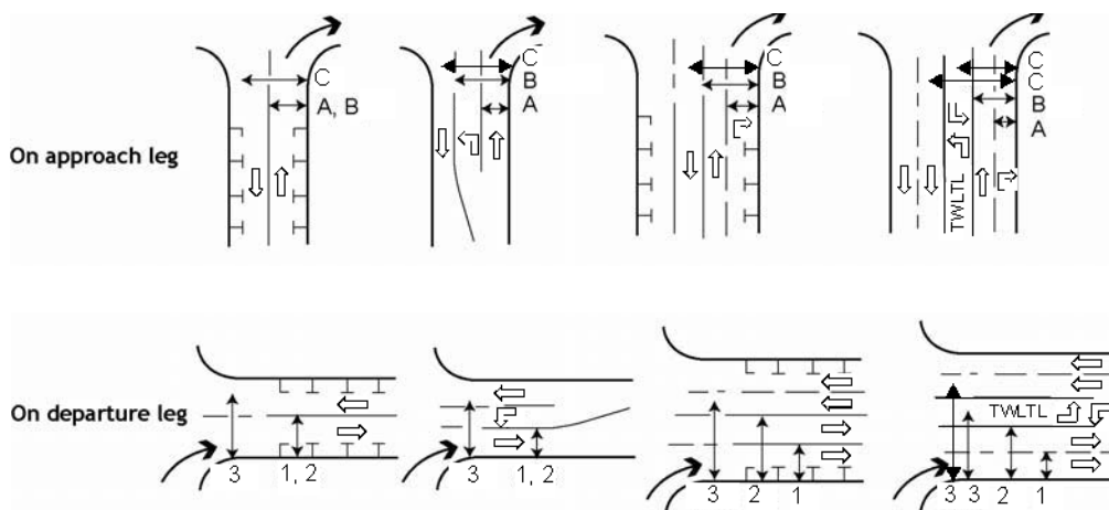
Figure 2.4 Effective Pavement width and effect on degree of encroachment 27
