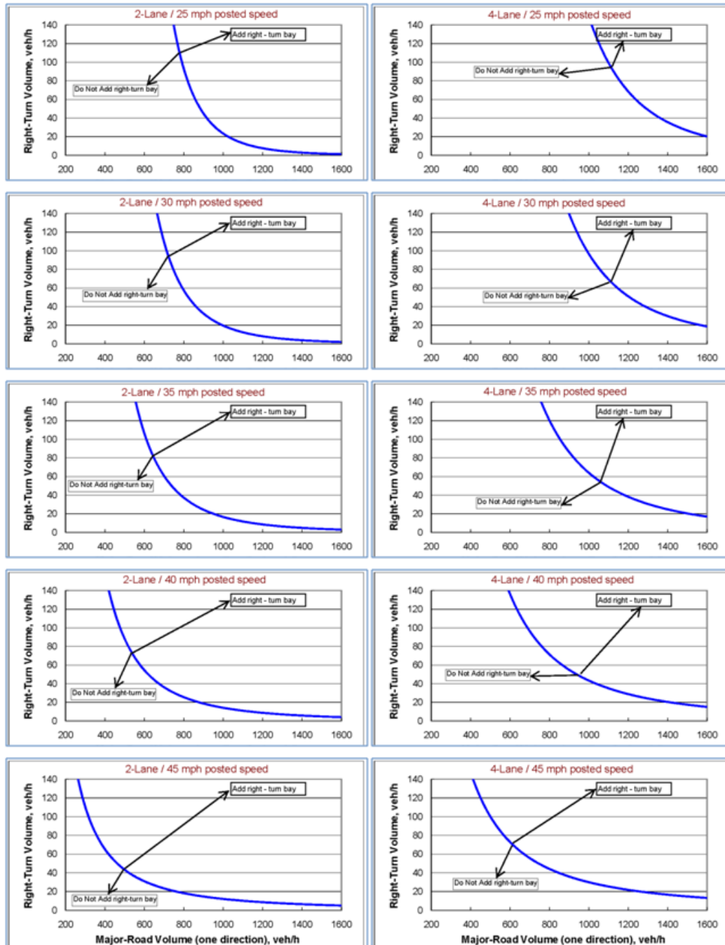
Figure 10.1 Guidelines for a Major-road Right-turn Bay at Urban Two-way Stop-controlled Intersections 72
