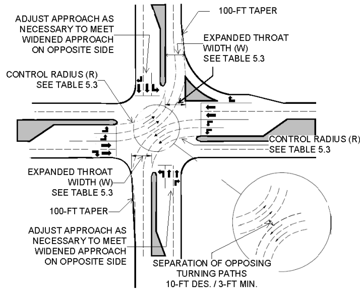
Figure 5.6 Dual Left Turn Lanes 65
