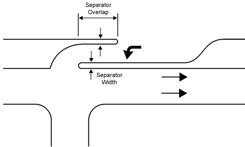
Figure 20.2 Separator Overlap for Directional Median Opening 86
