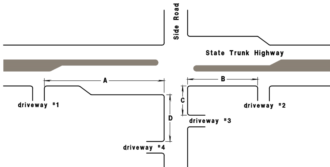
Figure 2.12 Intersection Marginal Corner Clearances 40 (See Table 2.7 )
