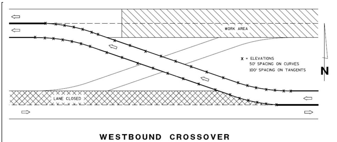
Figure 22.2 Westbound Crossover
